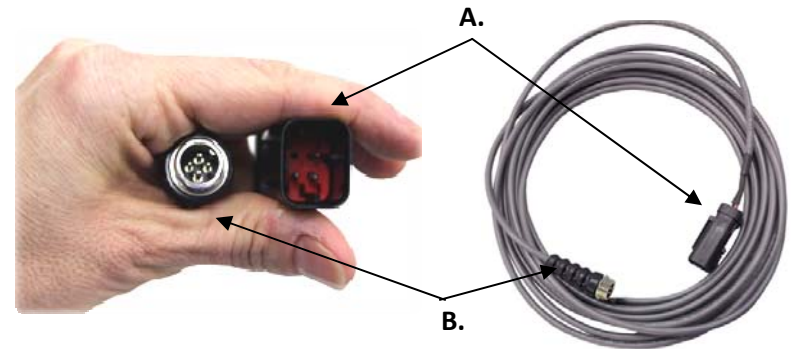
A. 4-pin male TE Connectivity/Tyco Connector B. 5-pin male OverView Connector
