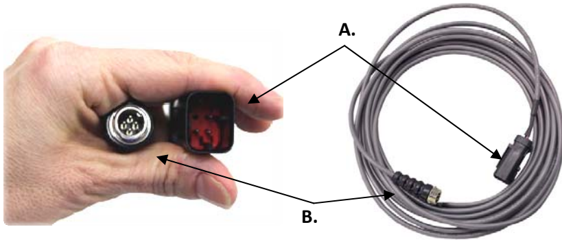
A. 4-pin male TE Connectivity/Tyco Connector B. 5-pin male OverView Connector
